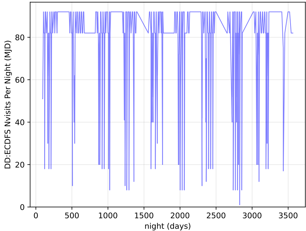
too_elab_heavy_r32_d2_gz_v3.4_10yrs all bands: DD:ECDFS Nvisits Per Night
