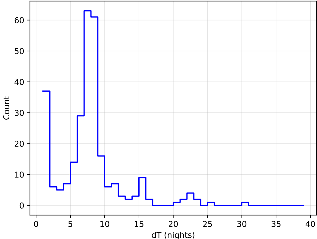
too_elab_heavy_r32_d2_gz_v3.4_10yrs all bands: DD:ECDFS Delta Nights Histogram
