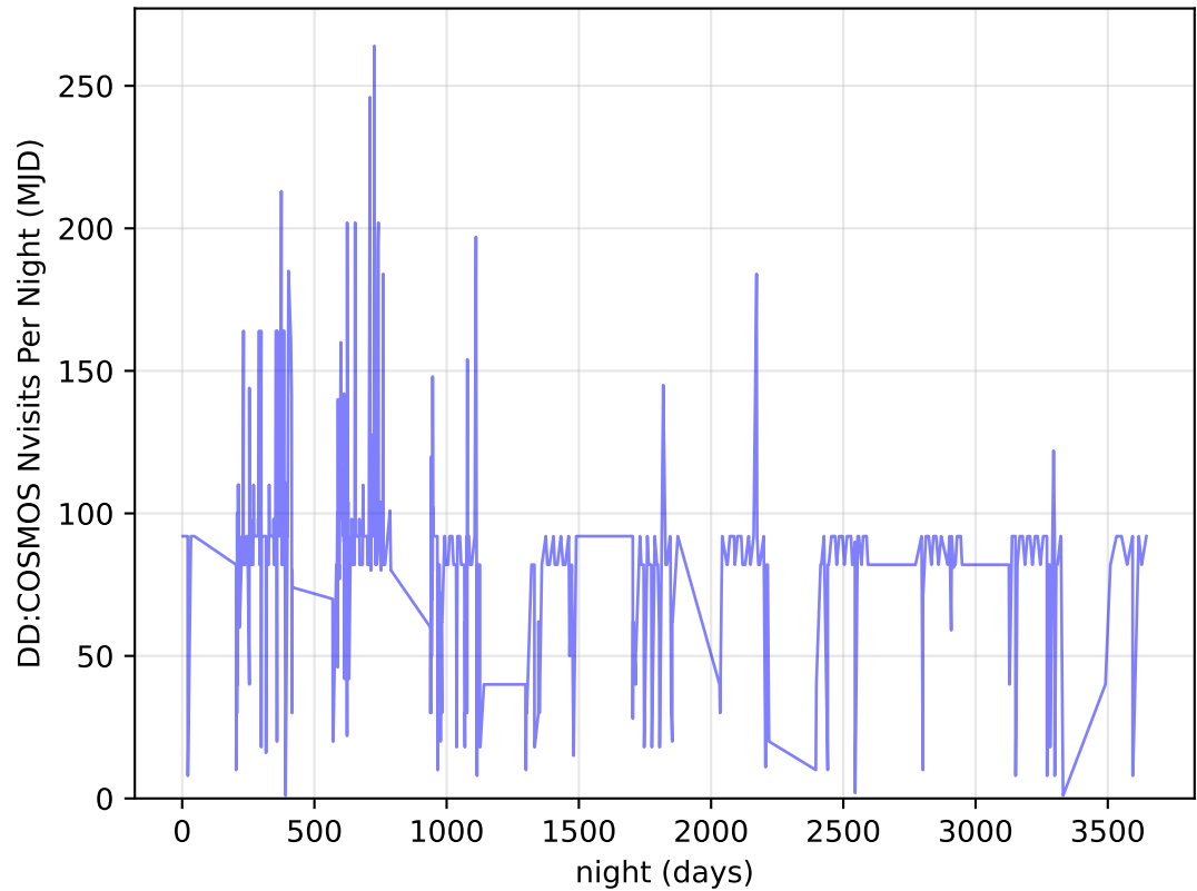
too_elab_heavy_r32_d2_gz_v3.4_10yrs all bands: DD:COSMOS Nvisits Per Night
