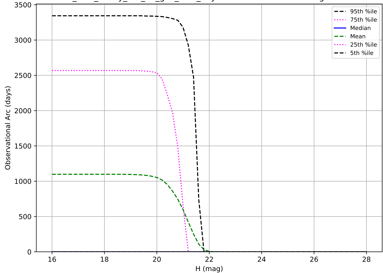
too_elab_heavy_r32_d2_griz_v3.4_10yrs: Observational Arc Length Vatira
