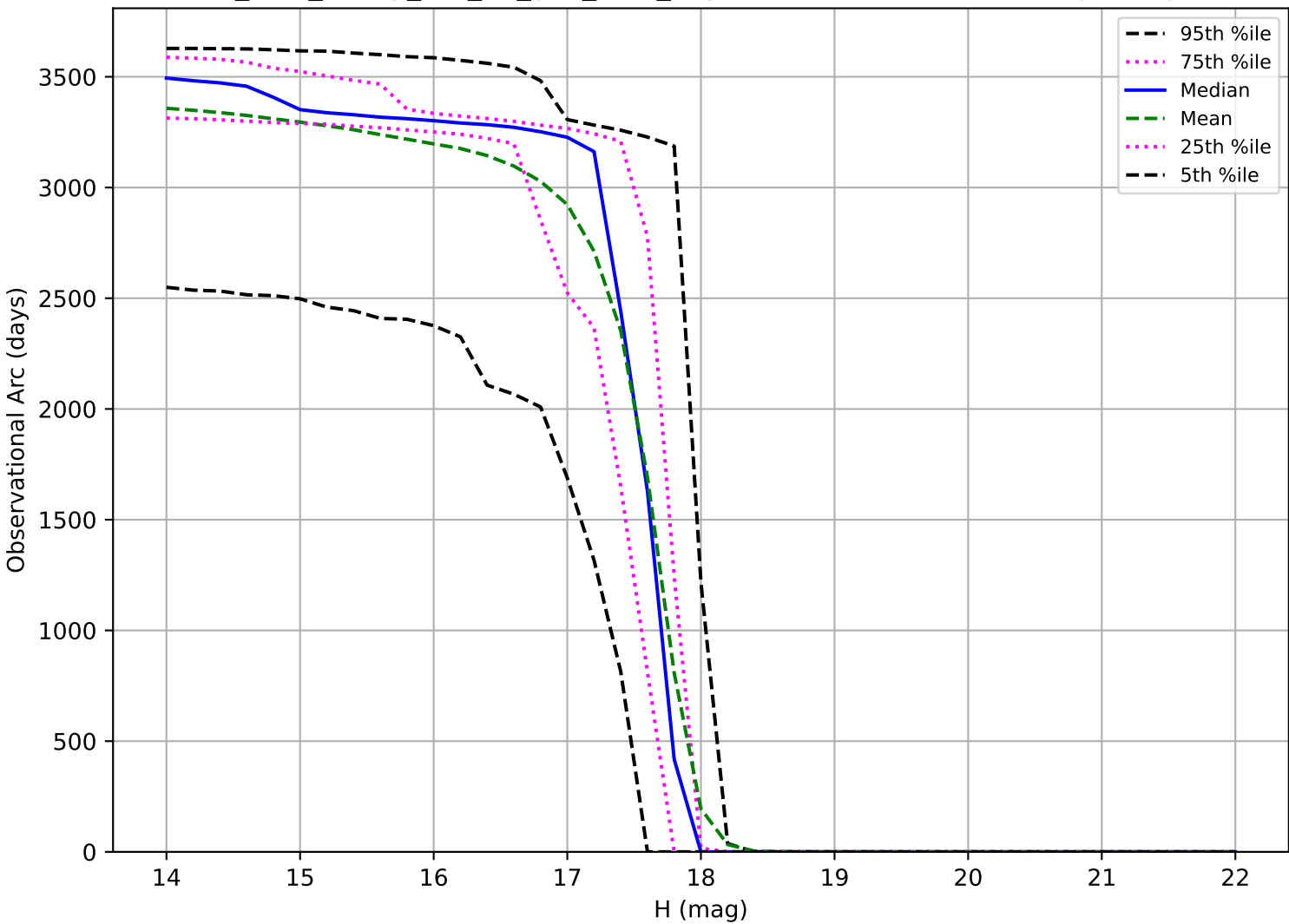
too_elab_heavy_r32_d2_griz_v3.4_10yrs: Observational Arc Length Trojan
