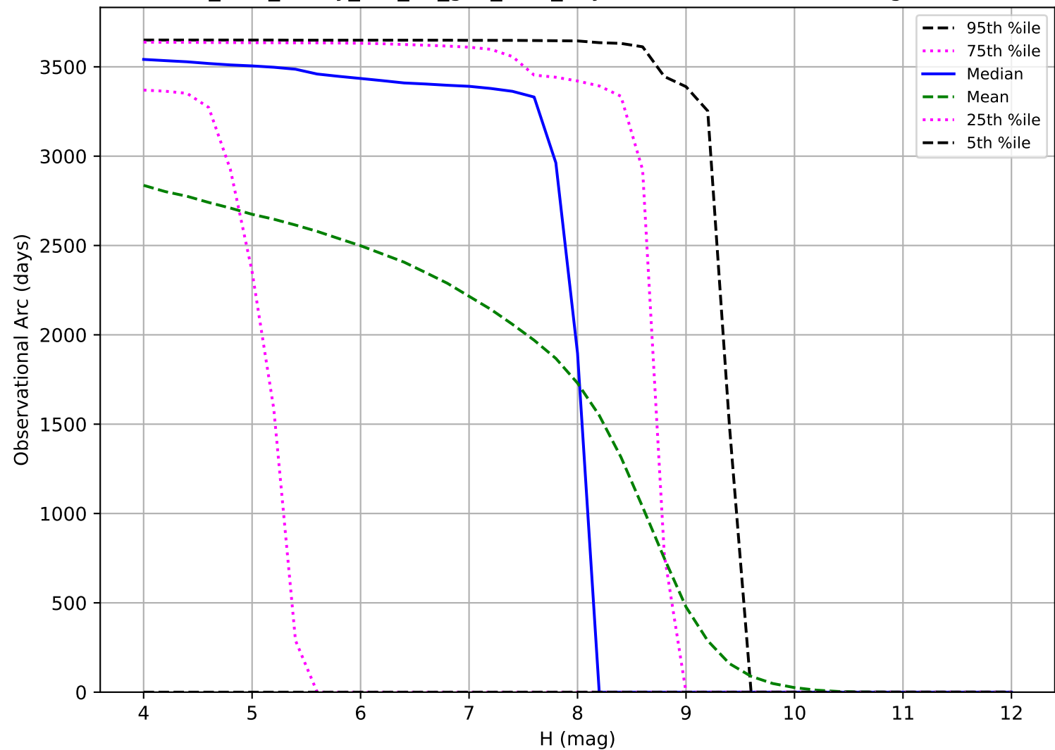
too_elab_heavy_r32_d2_griz_v3.4_10yrs: Observational Arc Length TNO
