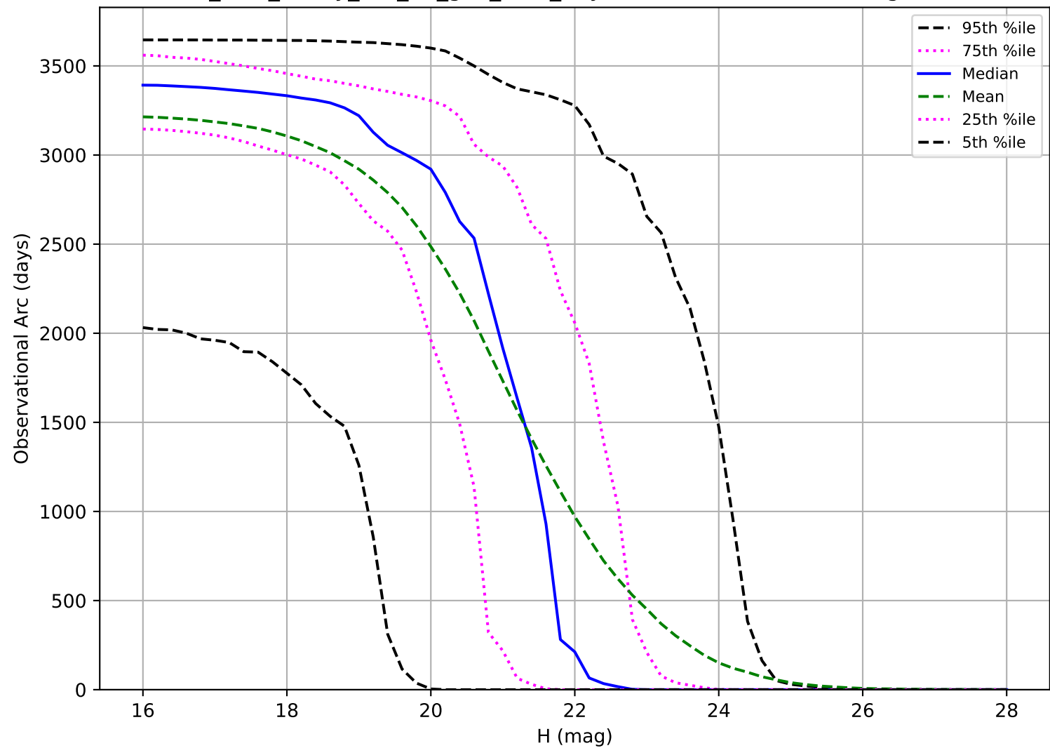
too_elab_heavy_r32_d2_griz_v3.4_10yrs: Observational Arc Length PHA
