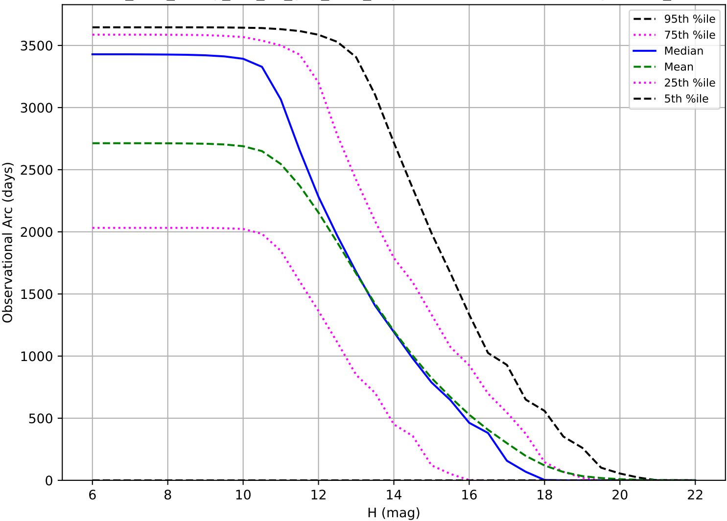
too_elab_heavy_r32_d2_griz_v3.4_10yrs: Observational Arc Length OCC_r5
