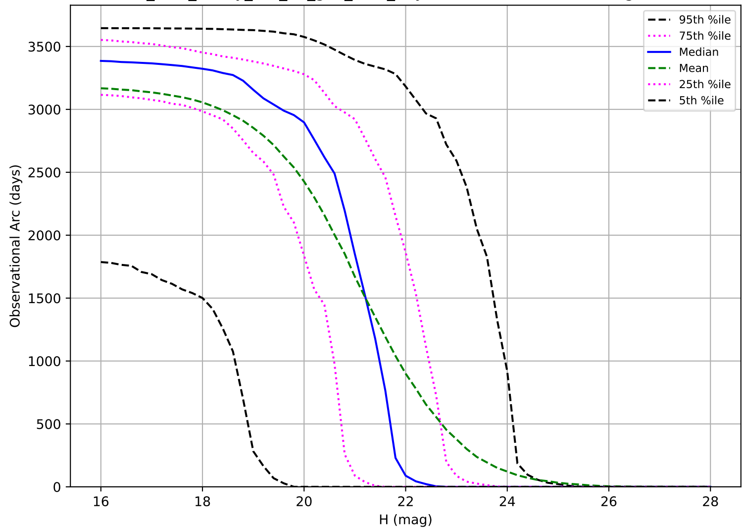
too_elab_heavy_r32_d2_griz_v3.4_10yrs: Observational Arc Length NEO
