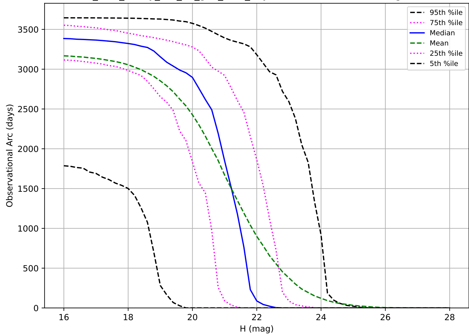
too_elab_heavy_r32_d2_griz_v3.4_10yrs: Observational Arc Length NEO
