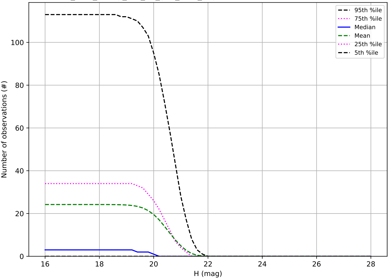
too_elab_heavy_r32_d2_griz_v3.4_10yrs: Number of observations Vatira
