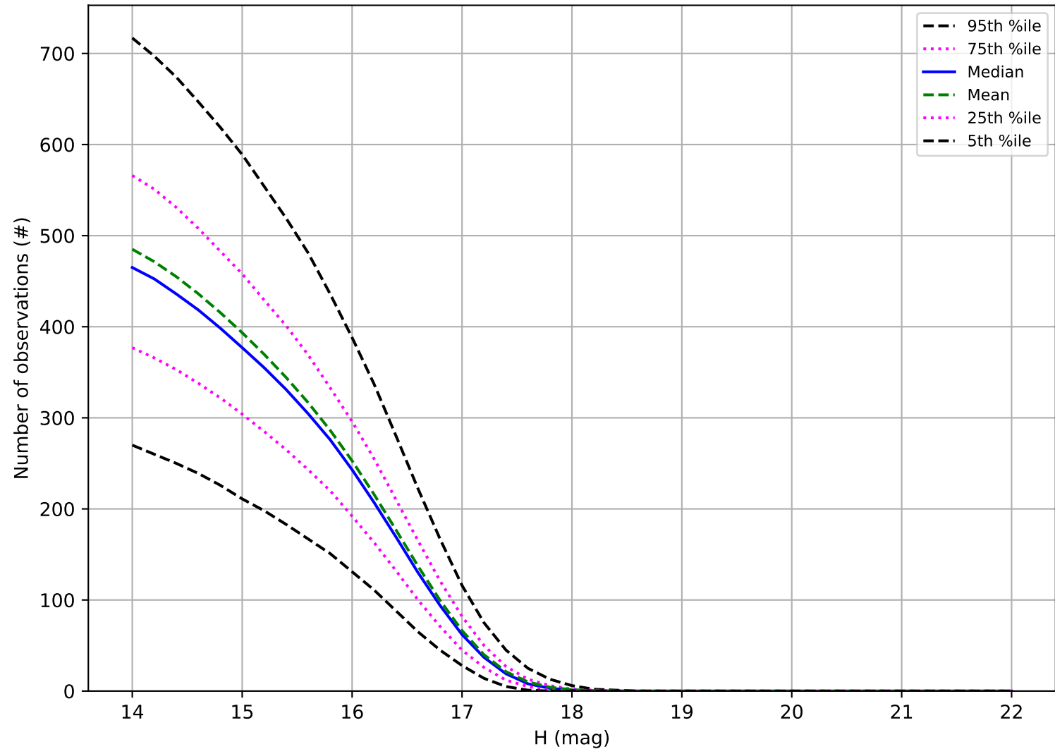
too_elab_heavy_r32_d2_griz_v3.4_10yrs: Number of observations Trojan
