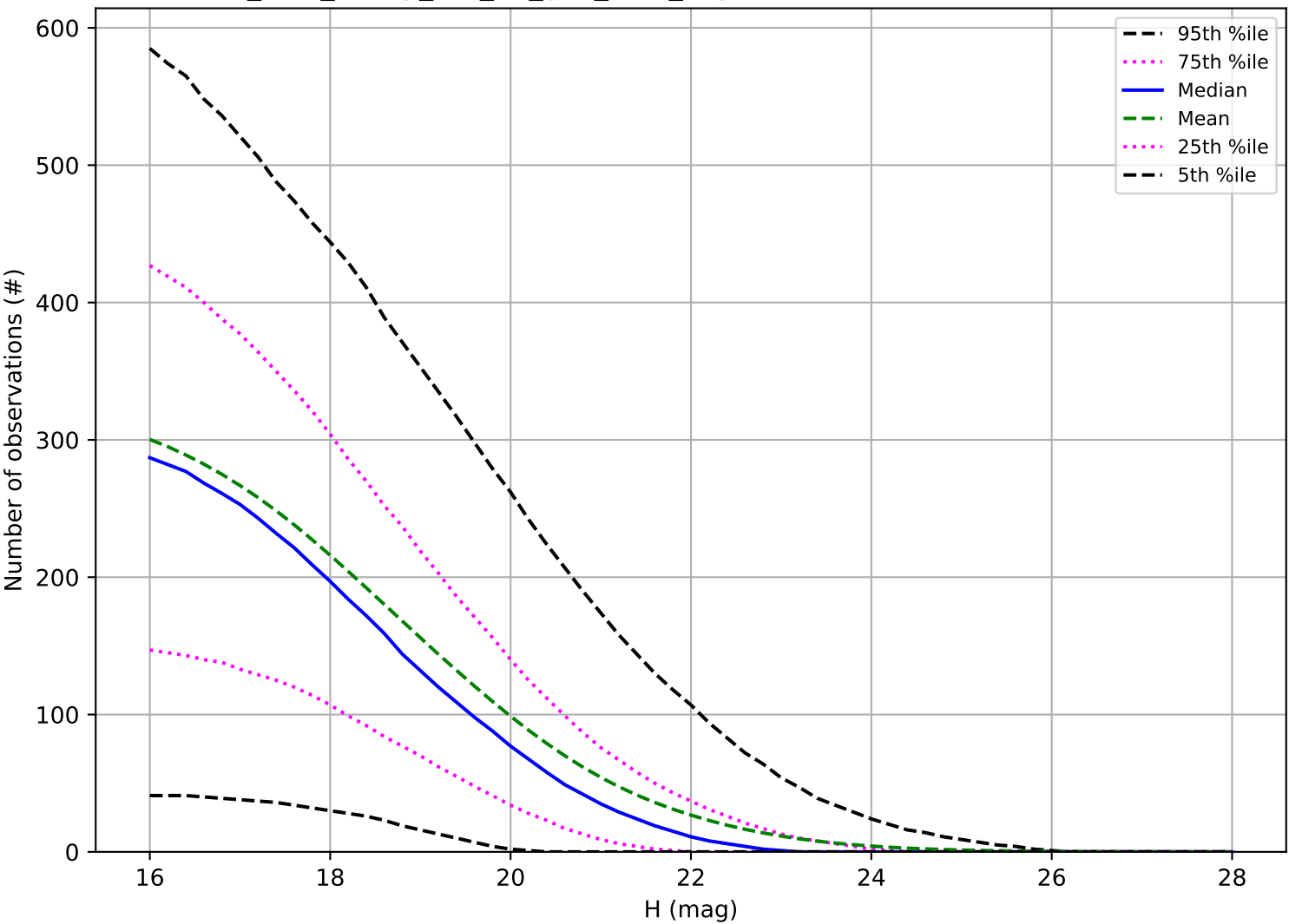
too_elab_heavy_r32_d2_griz_v3.4_10yrs: Number of observations PHA
