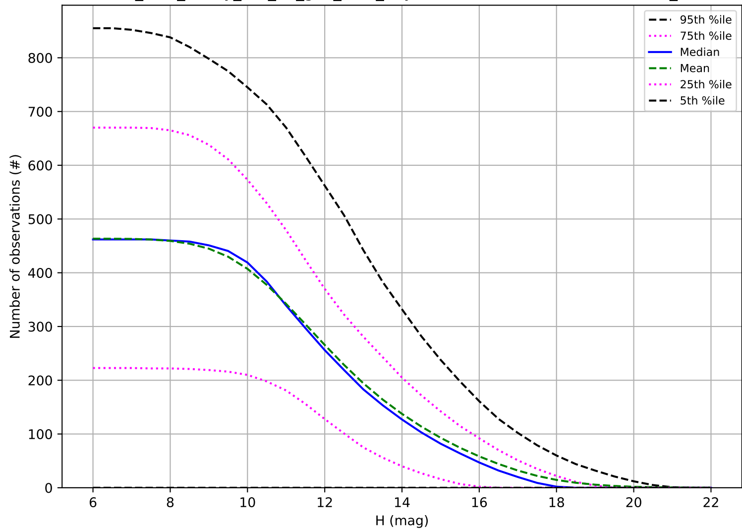
too_elab_heavy_r32_d2_griz_v3.4_10yrs: Number of observations OCC_r5
