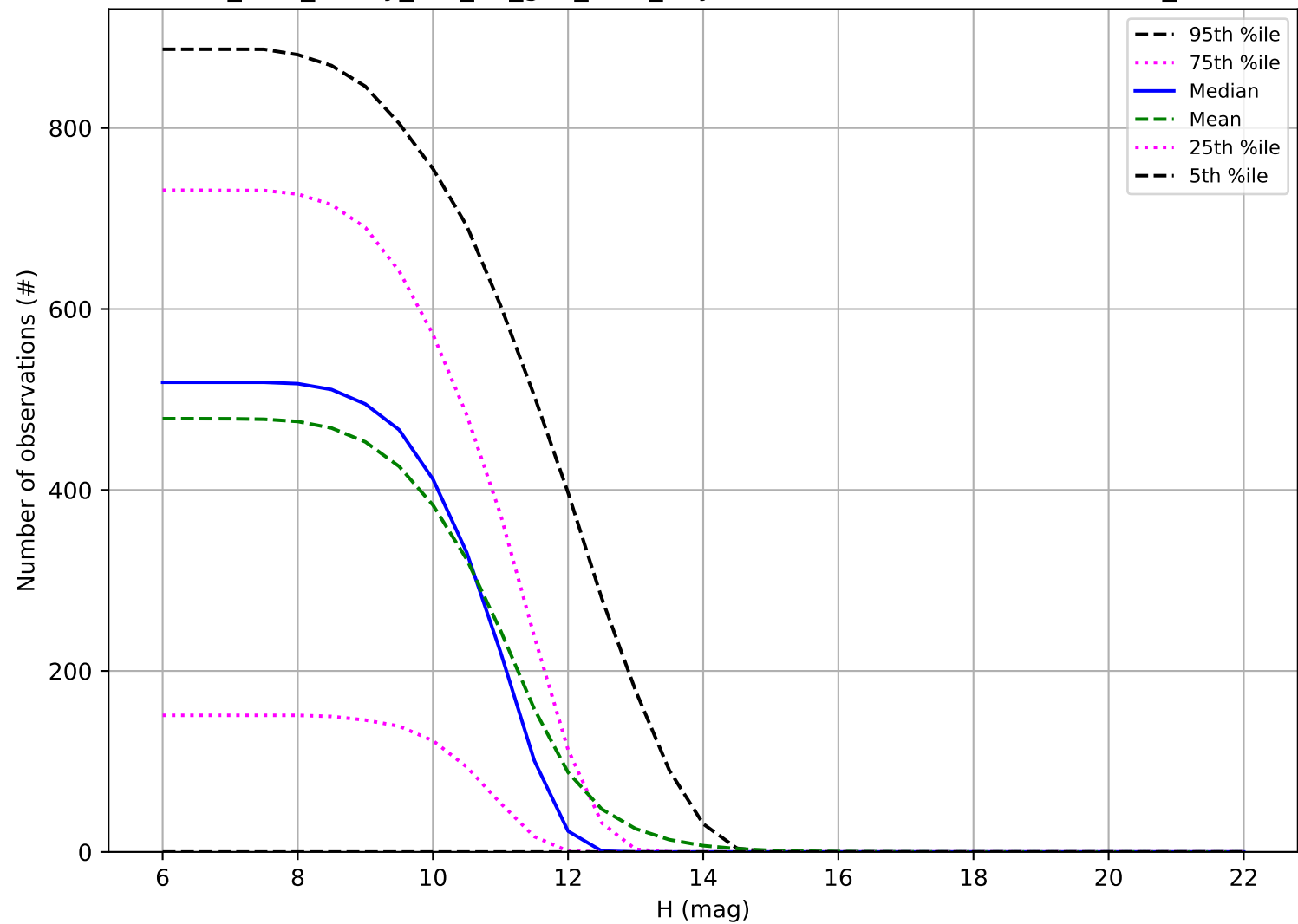
too_elab_heavy_r32_d2_griz_v3.4_10yrs: Number of observations OCC_r20
