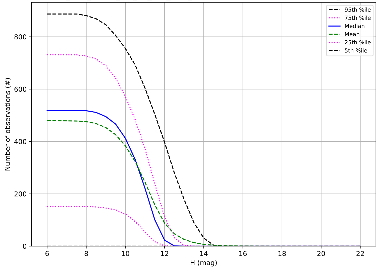
too_elab_heavy_r32_d2_griz_v3.4_10yrs: Number of observations OCC_r20
