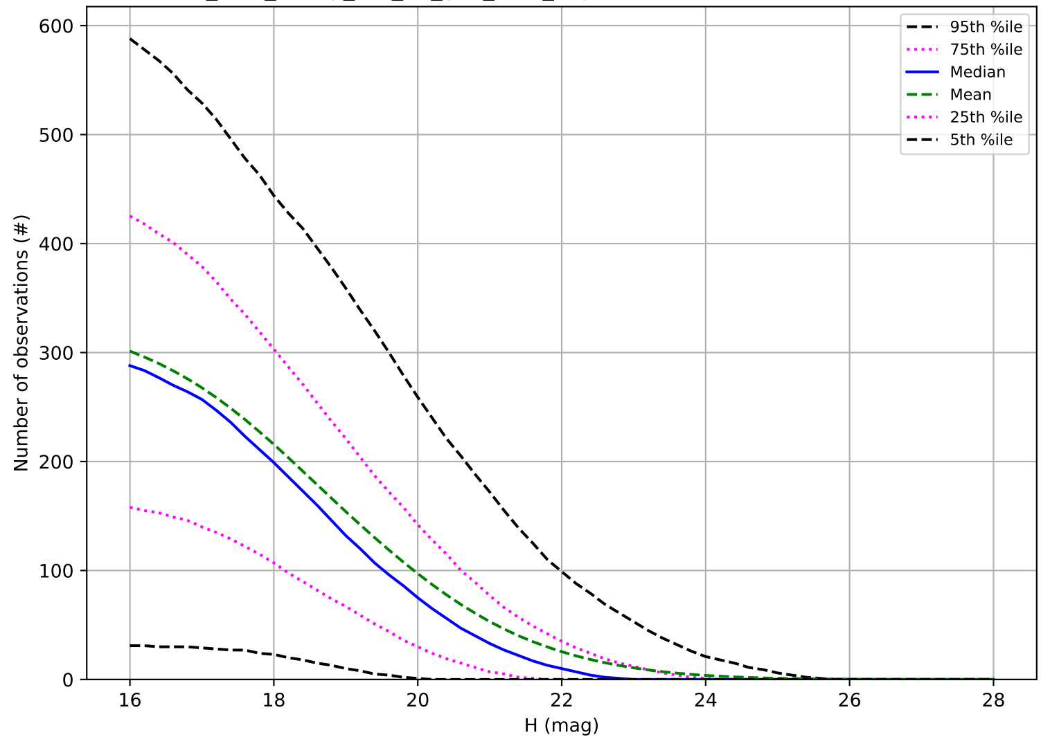
too_elab_heavy_r32_d2_griz_v3.4_10yrs: Number of observations NEO
