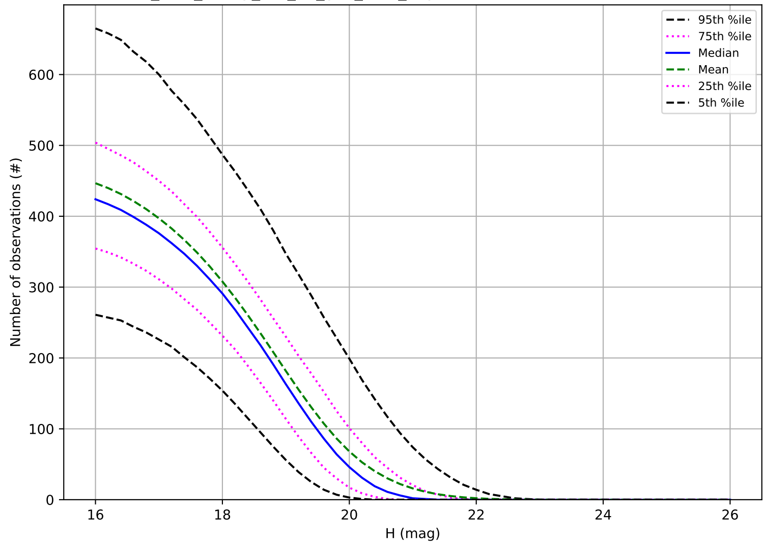
too_elab_heavy_r32_d2_griz_v3.4_10yrs: Number of observations MBA
