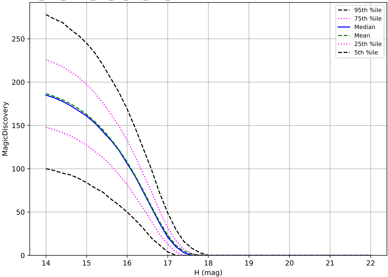
too_elab_heavy_r32_d2_griz_v3.4_10yrs: Trojan 6 detections in 60 nights detection loss
