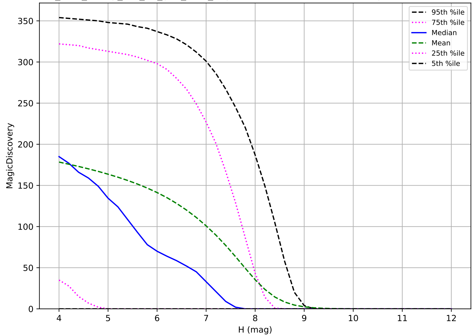
too_elab_heavy_r32_d2_griz_v3.4_10yrs: TNO 6 detections in 60 nights detection loss
