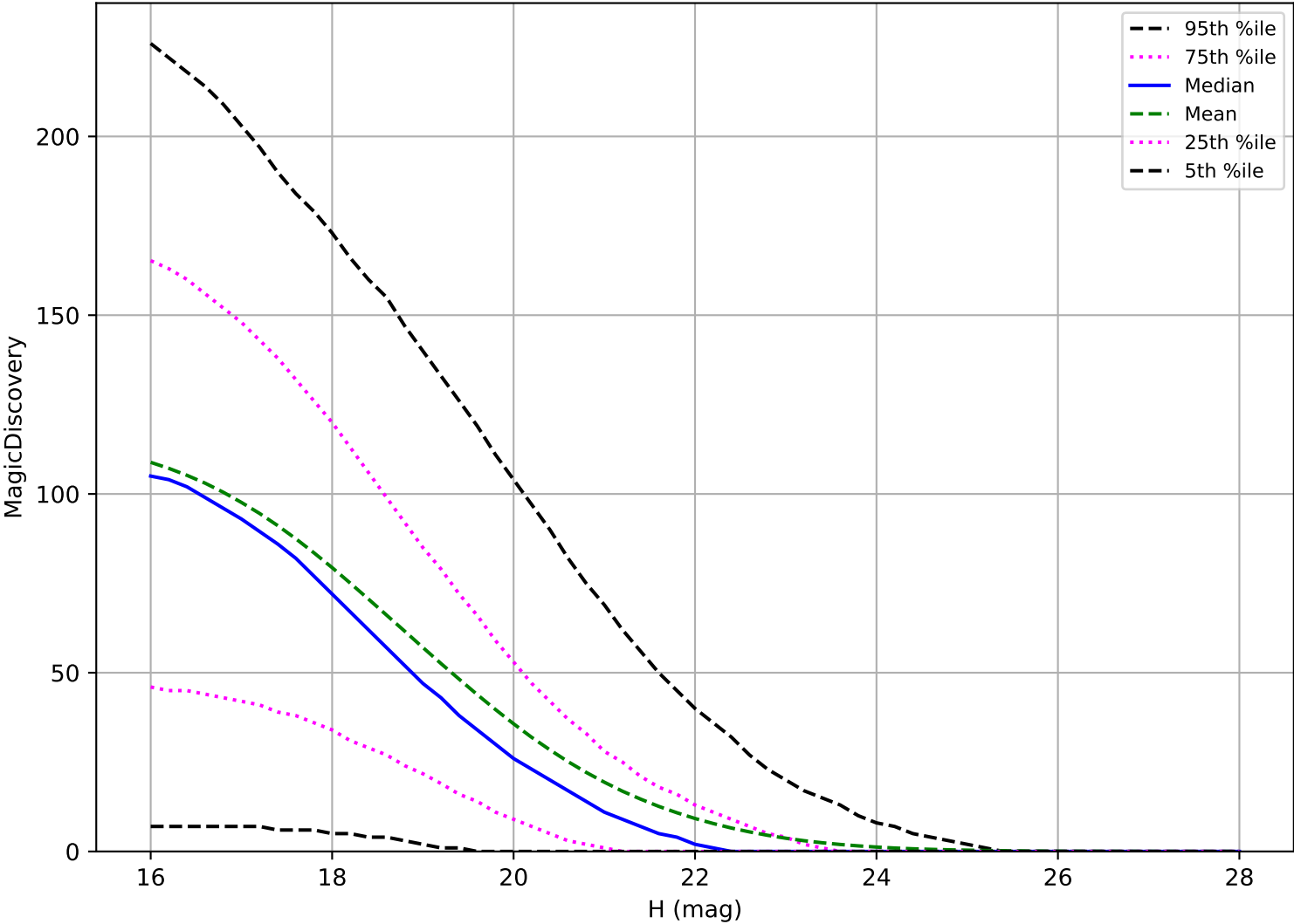
too_elab_heavy_r32_d2_griz_v3.4_10yrs: PHA 6 detections in 60 nights detection loss
