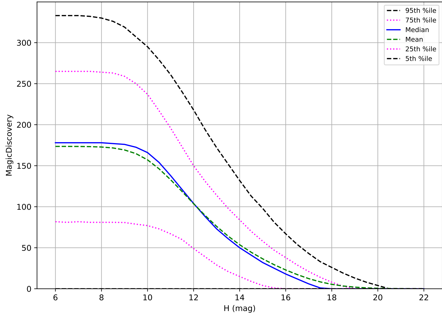
too_elab_heavy_r32_d2_griz_v3.4_10yrs: OCC_r5 6 detections in 60 nights detection loss
