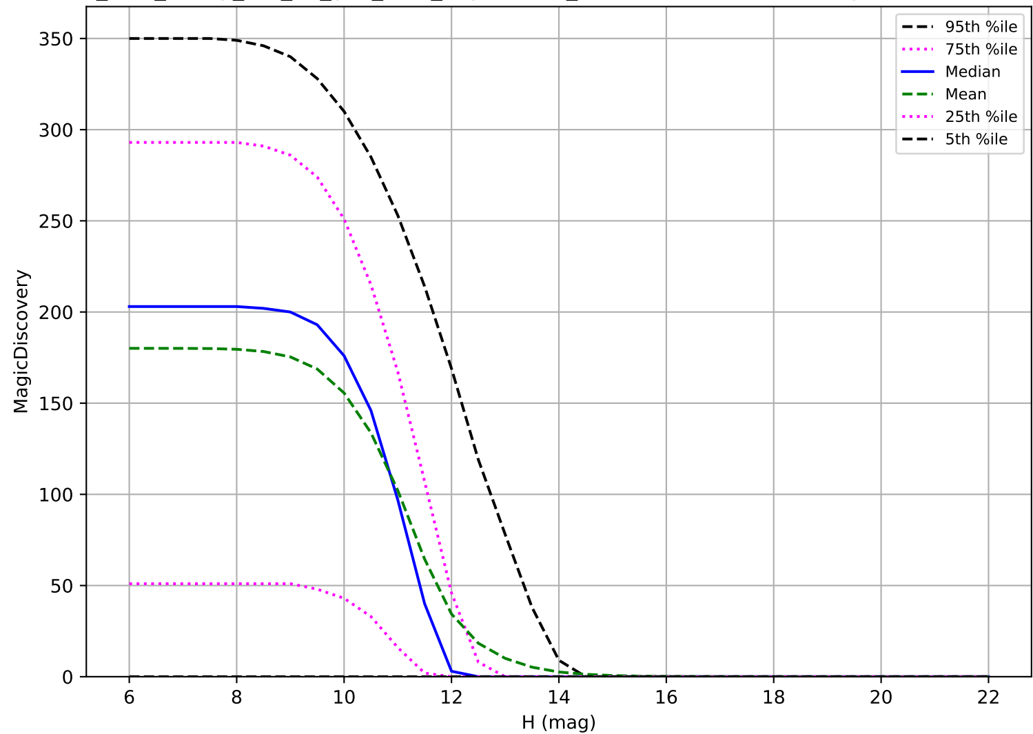
too_elab_heavy_r32_d2_griz_v3.4_10yrs: OCC_r20 6 detections in 60 nights detection loss
