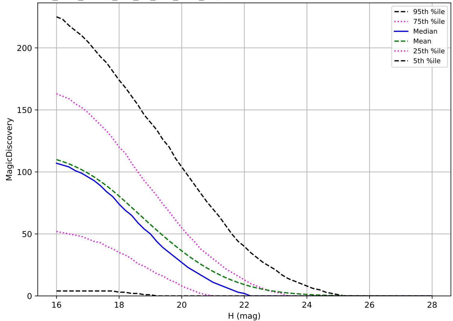
too_elab_heavy_r32_d2_griz_v3.4_10yrs: NEO 6 detections in 60 nights detection loss
