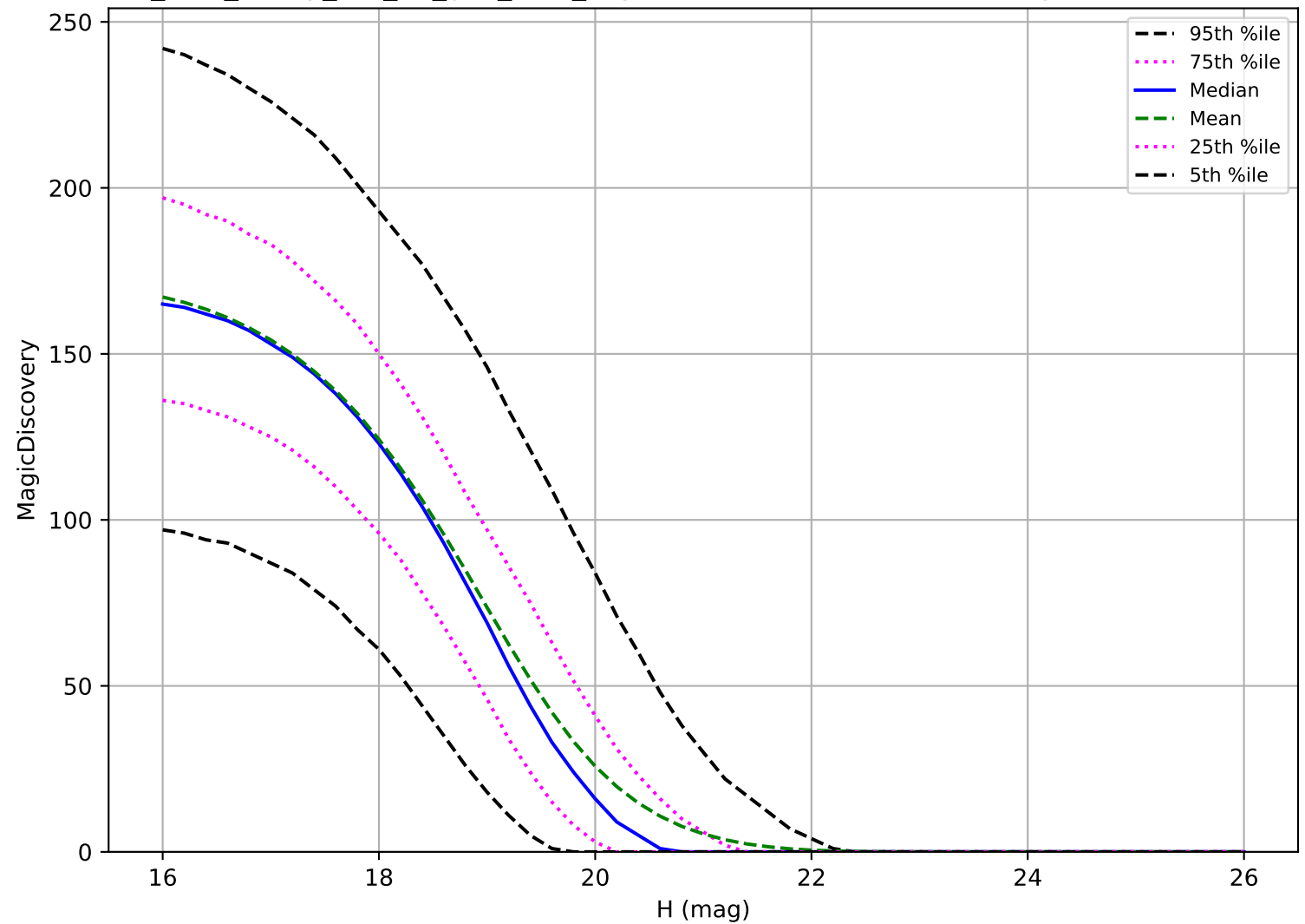
too_elab_heavy_r32_d2_griz_v3.4_10yrs: MBA 6 detections in 60 nights detection loss
