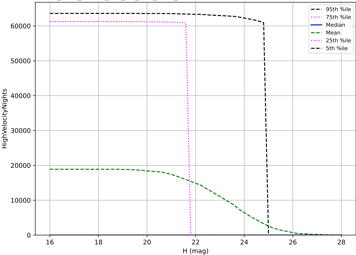
too_elab_heavy_r32_d2_griz_v3.4_10yrs: NEO High velocity pair detection loss
