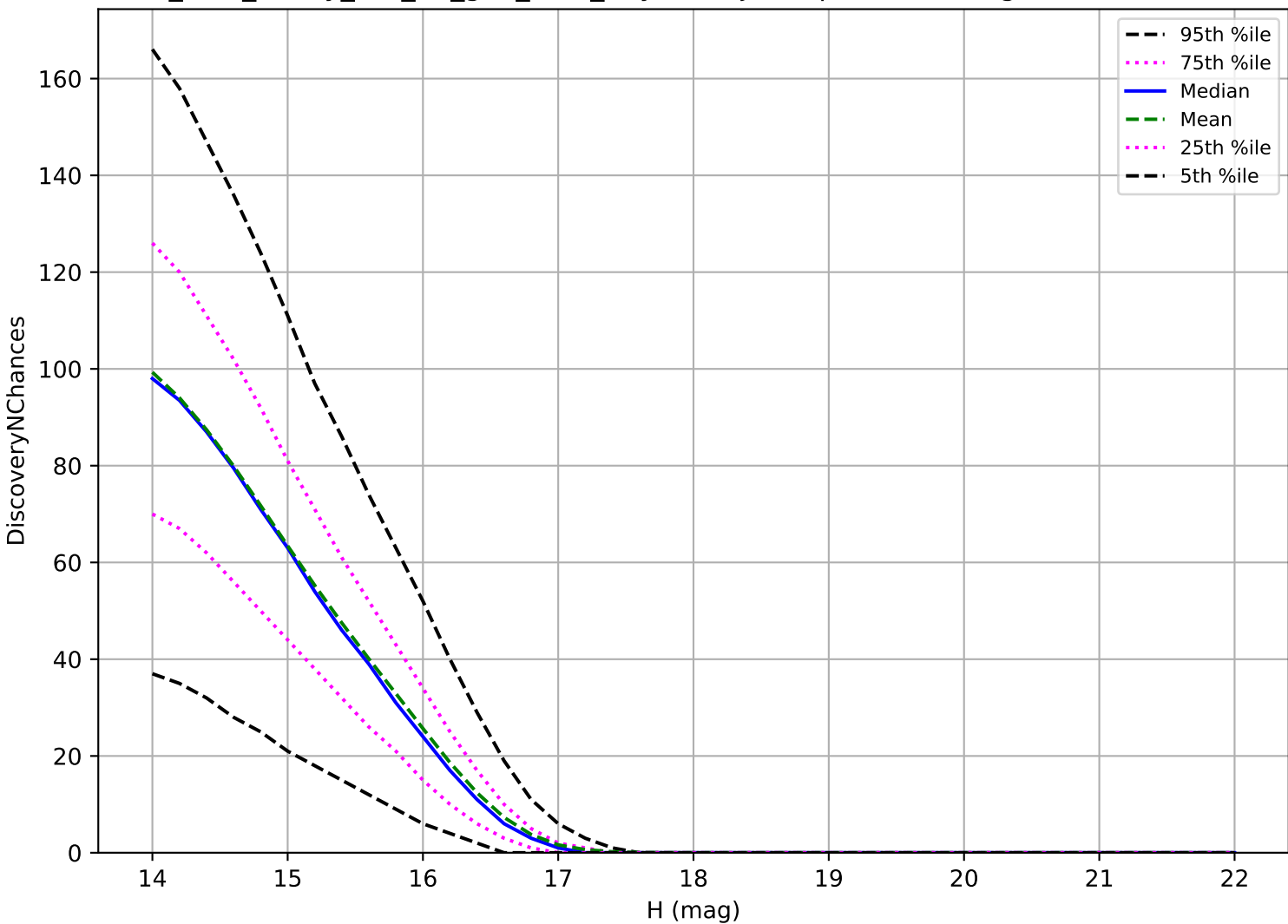
too_elab_heavy_r32_d2_griz_v3.4_10yrs: Trojan 3 pairs in 15 nights detection loss
