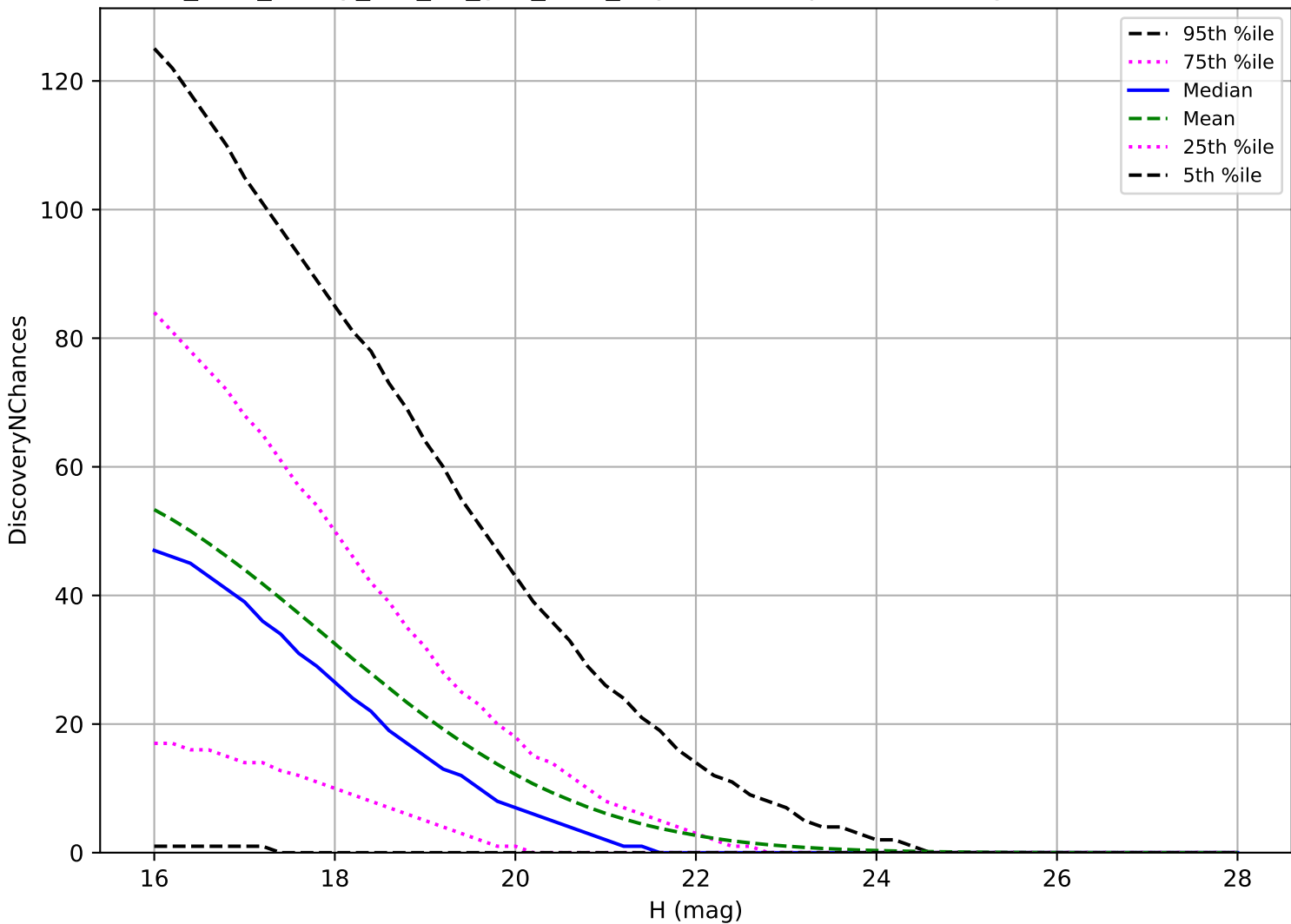
too_elab_heavy_r32_d2_griz_v3.4_10yrs: PHA 3 pairs in 15 nights detection loss
