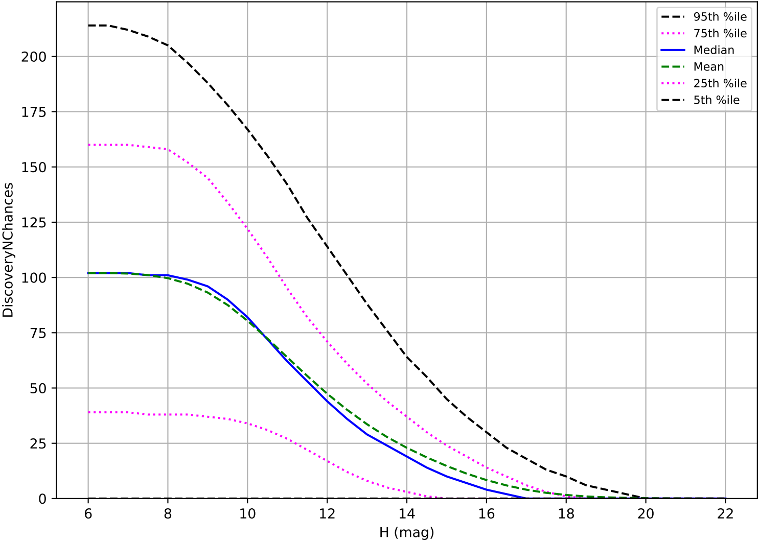
too_elab_heavy_r32_d2_griz_v3.4_10yrs: OCC_r5 3 pairs in 15 nights detection loss
