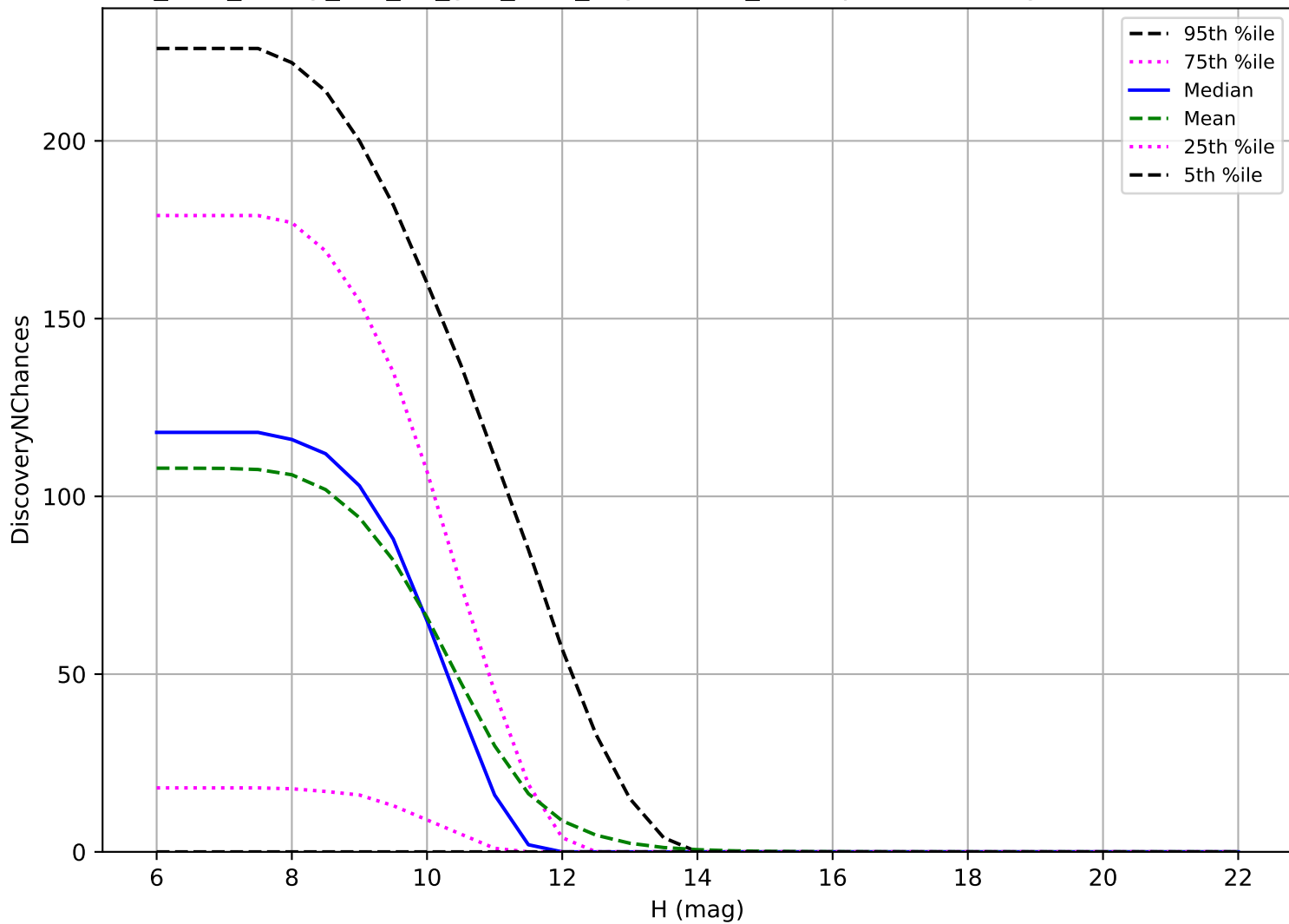
too_elab_heavy_r32_d2_griz_v3.4_10yrs: OCC_r20 3 pairs in 15 nights detection loss
