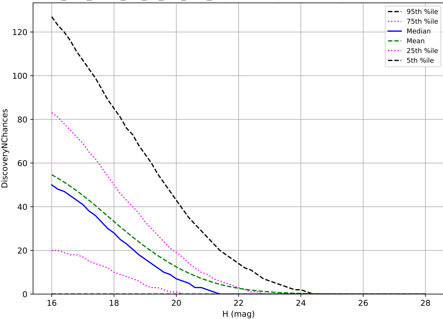
too_elab_heavy_r32_d2_griz_v3.4_10yrs: NEO 3 pairs in 15 nights detection loss
