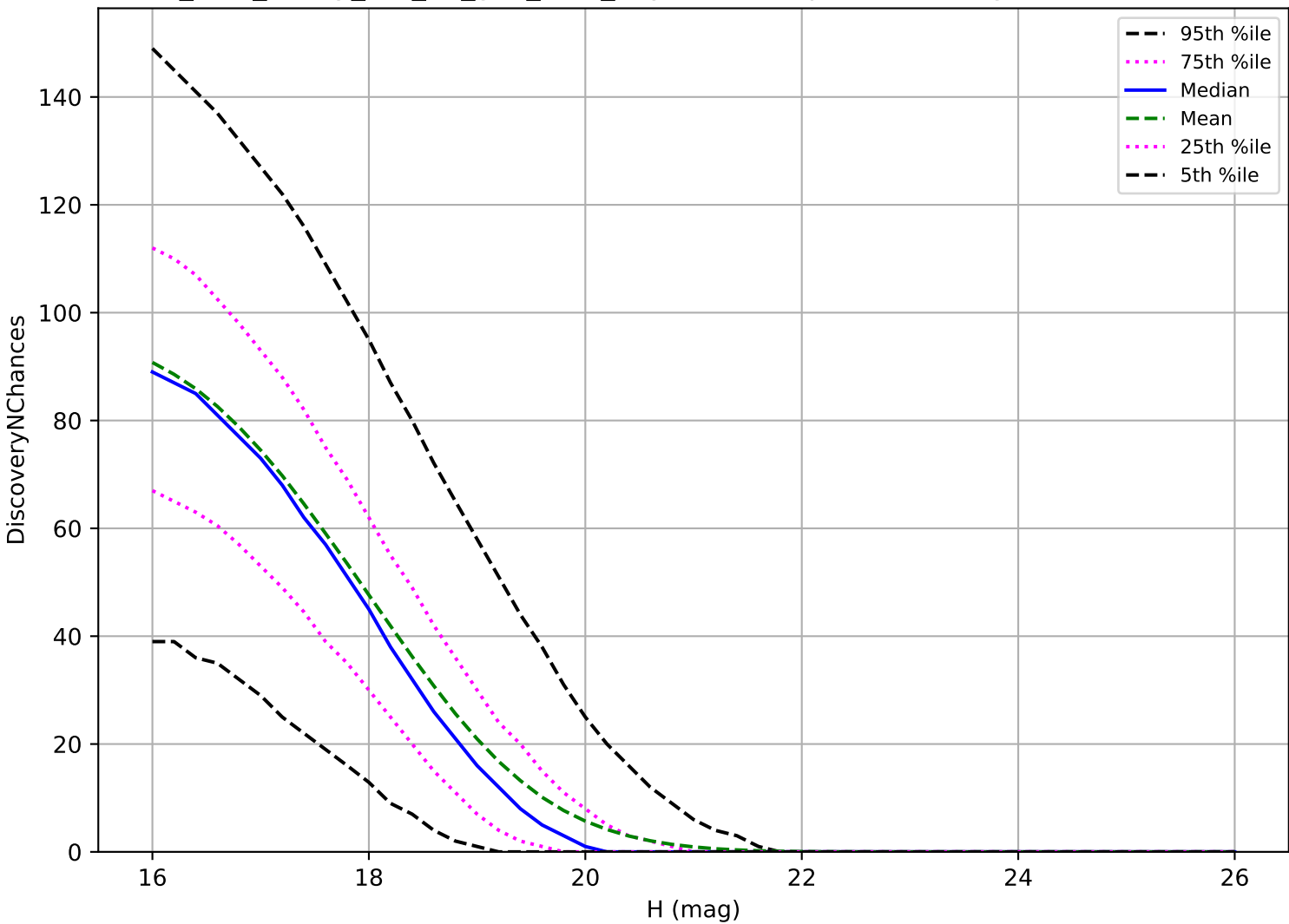
too_elab_heavy_r32_d2_griz_v3.4_10yrs: MBA 3 pairs in 15 nights detection loss
