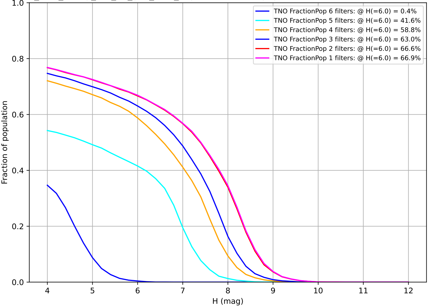
too_elab_heavy_r32_d2_griz_v3.4_10yrs: Fraction of population with colors in X filters TNO
