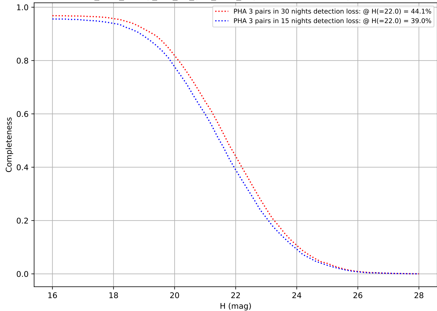
too_elab_heavy_r32_d2_griz_v3.4_10yrs: DifferentialCompleteness
