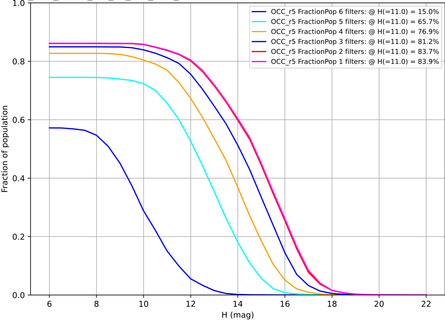
too_elab_heavy_r32_d2_griz_v3.4_10yrs: Fraction of population with colors in X filters OCC_r5
