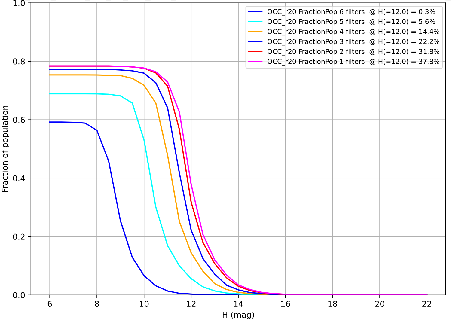
too_elab_heavy_r32_d2_griz_v3.4_10yrs: Fraction of population with colors in X filters OCC_r20
