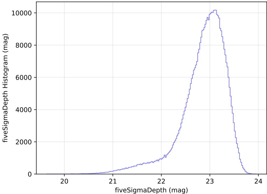
too_elab_heavy_r32_d2_griz_v3.4_10yrs z: fiveSigmaDepth Histogram
