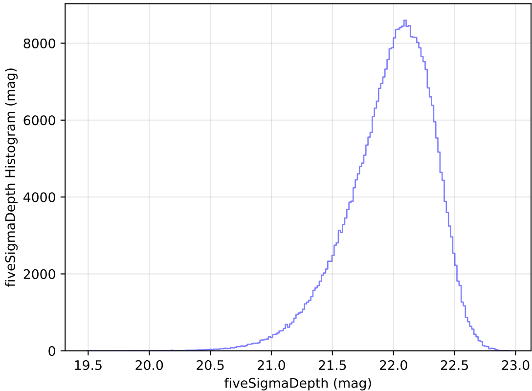
too_elab_heavy_r32_d2_griz_v3.4_10yrs y: fiveSigmaDepth Histogram
