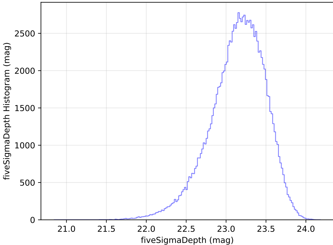
too_elab_heavy_r32_d2_griz_v3.4_10yrs u: fiveSigmaDepth Histogram
