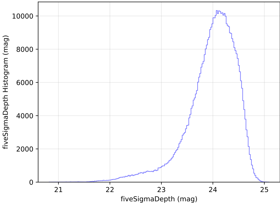
too_elab_heavy_r32_d2_griz_v3.4_10yrs r: fiveSigmaDepth Histogram
