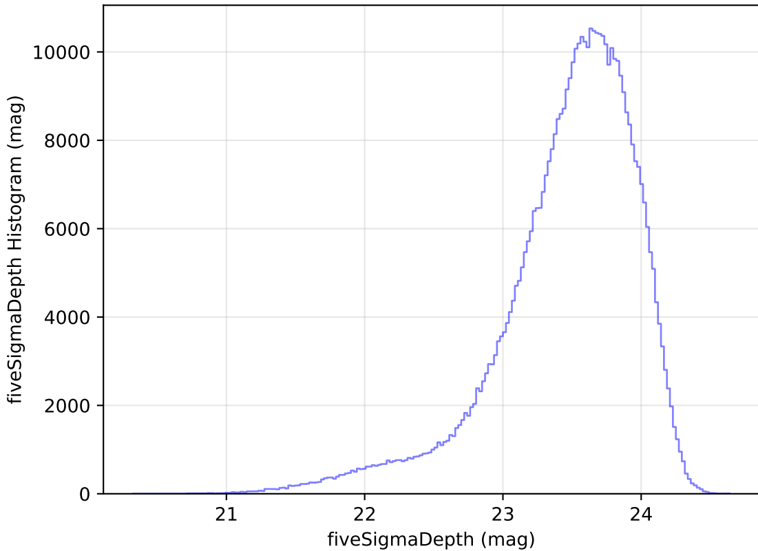
too_elab_heavy_r32_d2_griz_v3.4_10yrs i: fiveSigmaDepth Histogram
