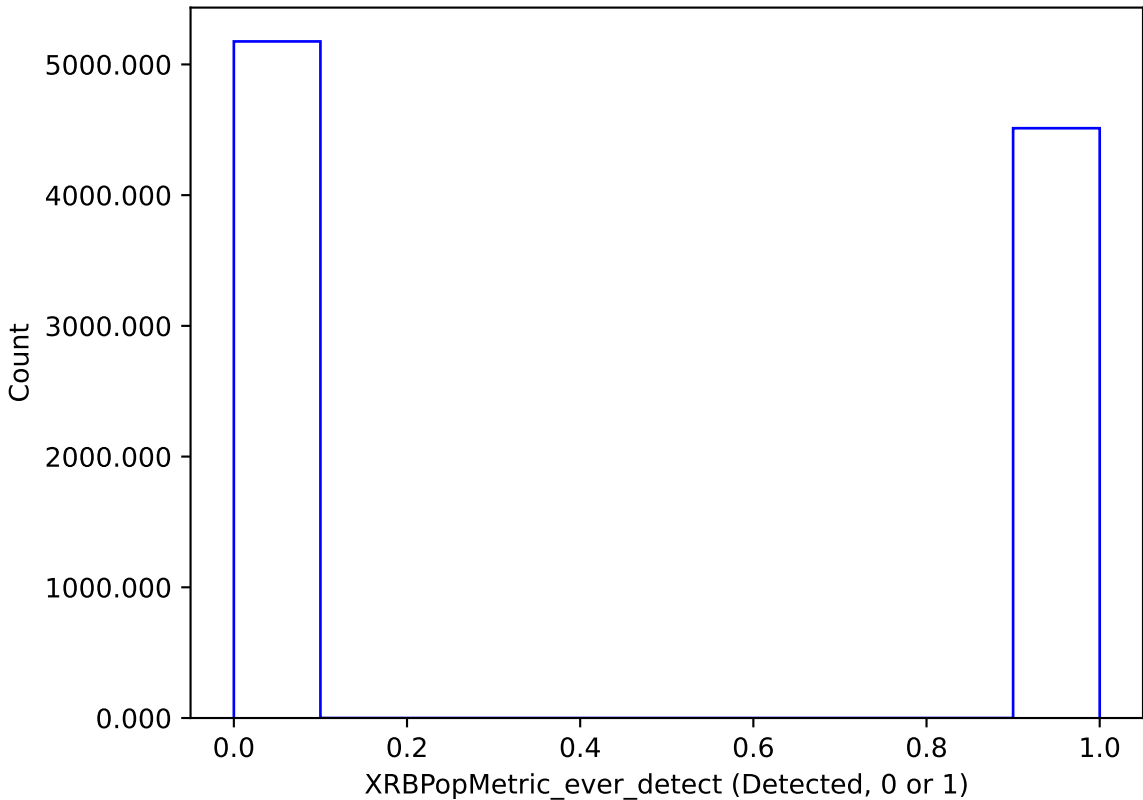
too_elab_heavy_r32_d2_griz_v3.4_10yrs : XRBPoMetric_ever_detect
