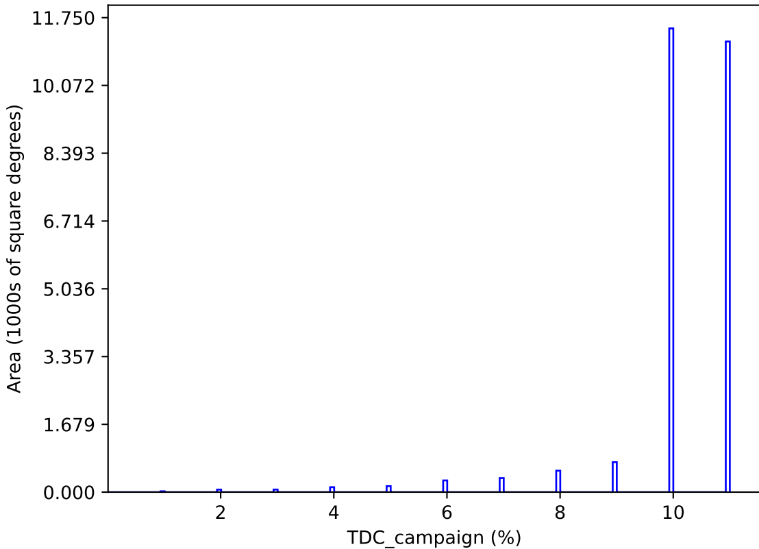
too_elab_heavy_r32_d2_griz_v3.4_10yrs : TDC_campaign
