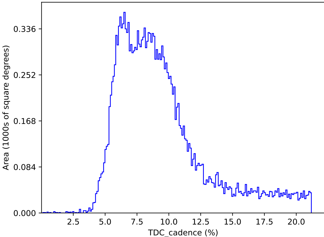
too_elab_heavy_r32_d2_griz_v3.4_10yrs : TDC_cadence
