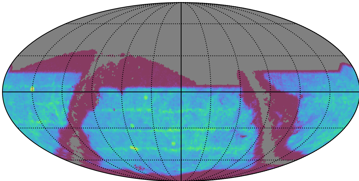
too_elab_heavy_r32_d2_griz_v3.4_10yrs : SNSLMetric
