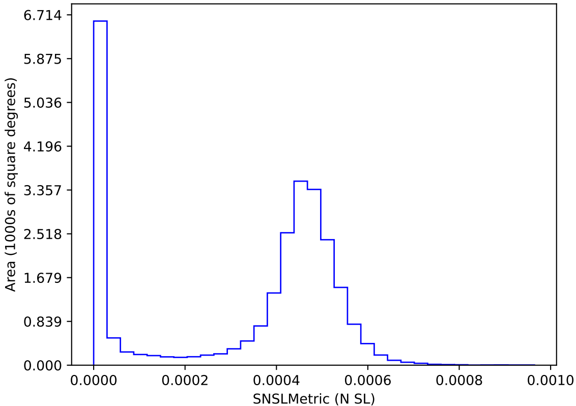
too_elab_heavy_r32_d2_griz_v3.4_10yrs : SNSLMetric
