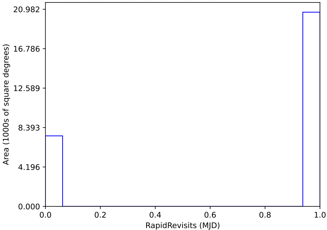
too_elab_heavy_r32_d2_griz_v3.4_10yrs : RapidRevisits
