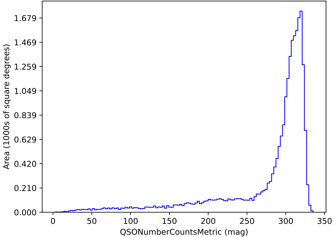
too_elab_heavy_r32_d2_griz_v3.4_10yrs u band and non-DD: QSONumberCountsMetric
