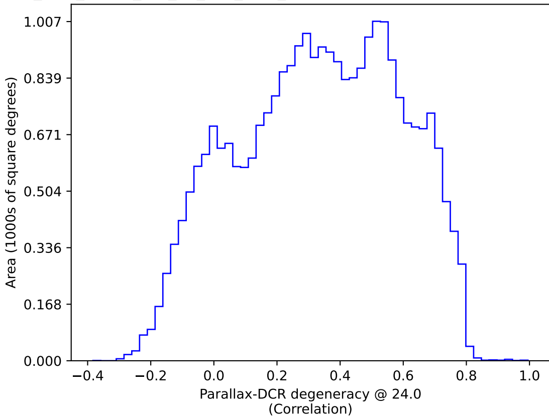
too_elab_heavy_r32_d2_griz_v3.4_10yrs : Parallax-DCR degeneracy @ 24.0
