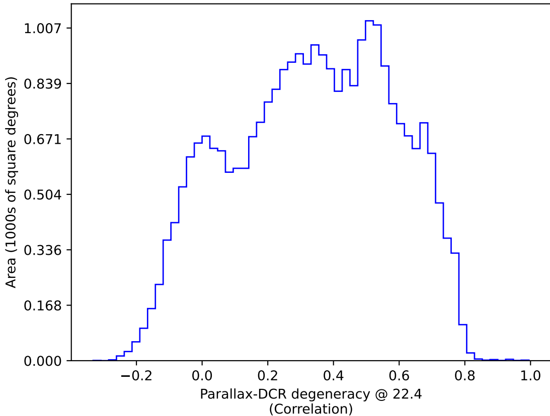
too_elab_heavy_r32_d2_griz_v3.4_10yrs : Parallax-DCR degeneracy @ 22.4
