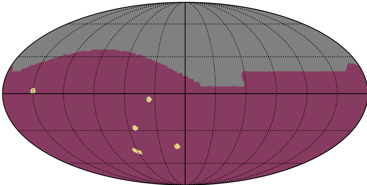
too_elab_heavy_r32_d2_griz_v3.4_10yrs : NumberOfQuickRevisits
