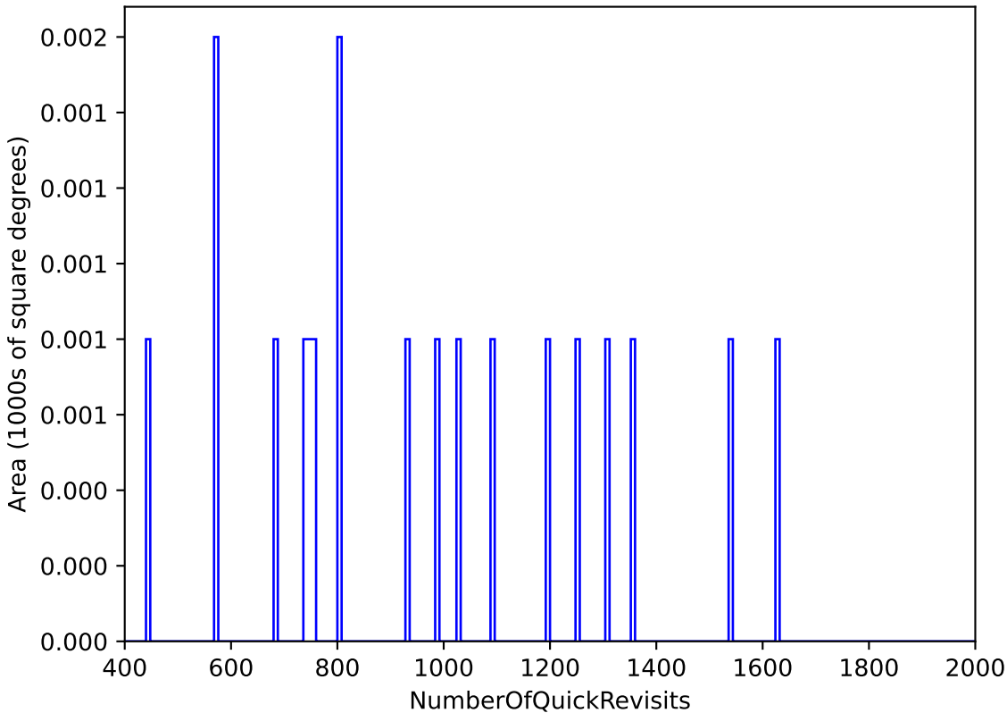
too_elab_heavy_r32_d2_griz_v3.4_10yrs : NumberOfQuickRevisits
